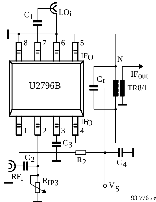
Figure 12. Application circuit
