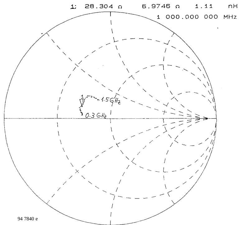
Figure 10. S11 RF input impedance
